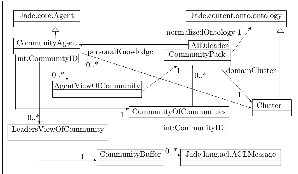
Fig. 1. UML Class diagram of the prototype.
